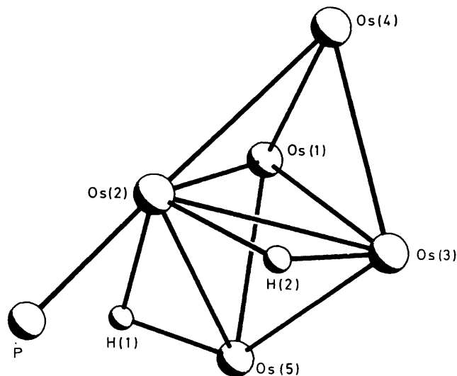
Figure 4. The core geometry of [Os 5 H 2 (CO) 14 (PEt 3 )] (12) showing the calculated positions of the hydrides
