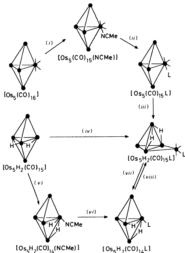
Scheme 2. (i) Me 3 NO, MeCN, CH 2 Cl 2 , room temperature (r.t.); (ii) L = P(OMe) 3 , PPh 3 , or P(OPh) 3 , r.t., CH 2 Cl 2 , 3–4 h; (iii) for L = P(OMe) 3 , H - /H + , CH 2 Cl 2 , r.t.; (iv) L = P(OMe) 3 , PPh 3 , or PEt 3 , CH 2 Cl 2 , reflux, 20 h; (v) Me 3 NO, MeCN, CH 2 Cl 2 , -78 °C; (vi) L = P(OMe) 3 , PPh 3 , or PEt 3 , CH 2 Cl 2 , r.t.; (vii) heat, n-octane, 1 h, -CO; (viii) CO (40 atm, 50 °C, 5 h)
