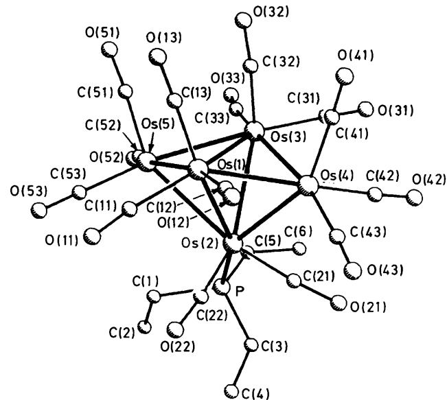
Figure 3. The molecular structure of [Os 5 H 2 (CO) 14 (PEt 3 )] (12)
